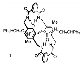
Figure 1. Rotaxane 1 used in this study.
