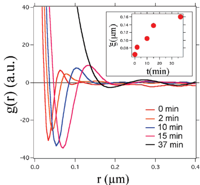
Figure 3. Evolution of the height–height correlation function extracted from the AFM images in Figure 2, showing both the increase and the shift in spatial correlations (height and position of the first maximum). Inset shows the evolution of the correlation length, viz. the position of the first maximum.
